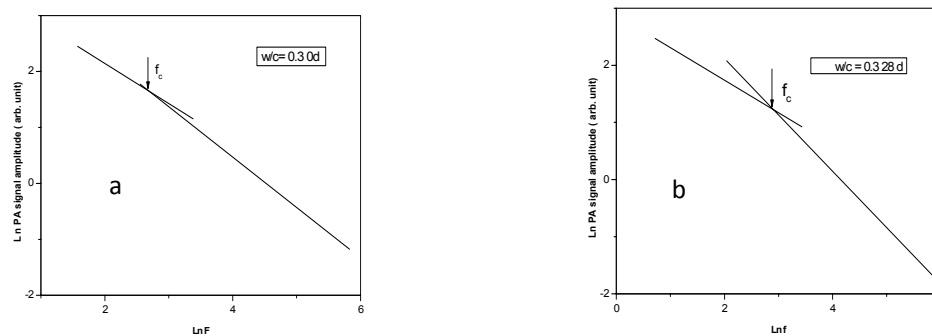
Figure 1. Variation of Ln PA amplitude with Ln of the modulation frequency for w/c = 0.3 at 0 d (a) and after one month (b).
